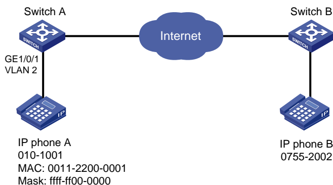
Figure 20 Network diagram
