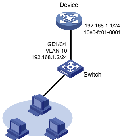
Figure 25 Network diagram
