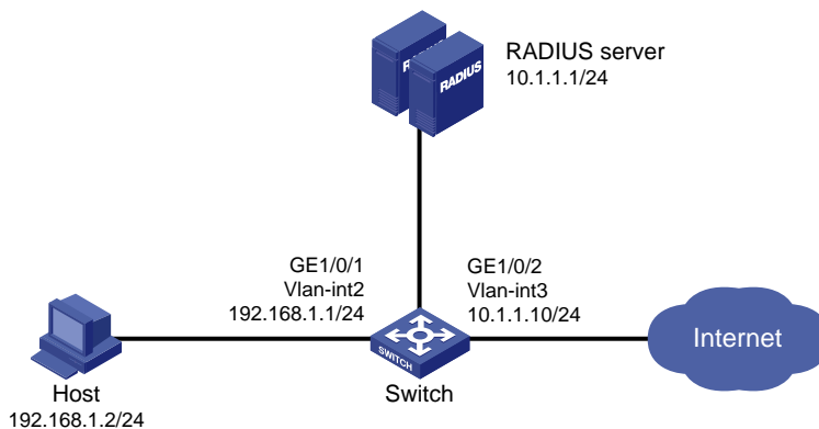
Figure 44 Network diagram
