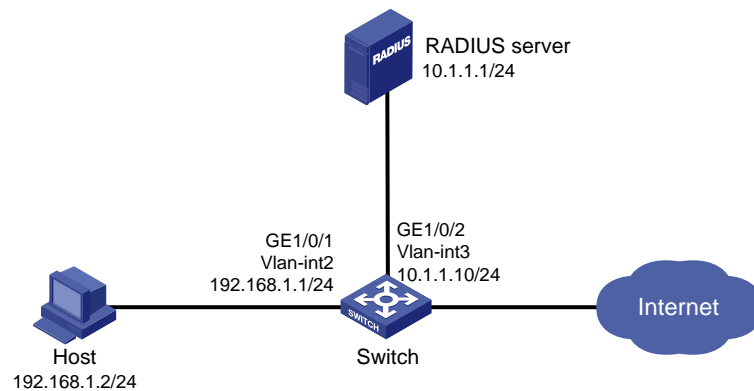
Figure 41 Network diagram
