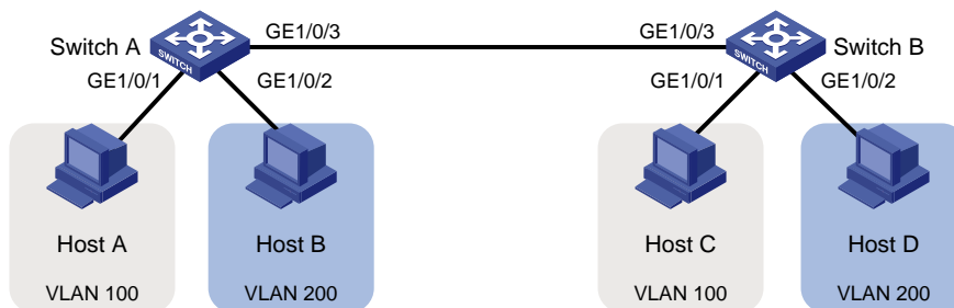
Figure 19 Network diagram
