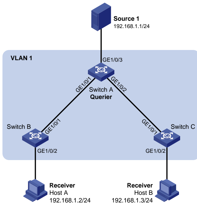
Figure 34 Network diagram
