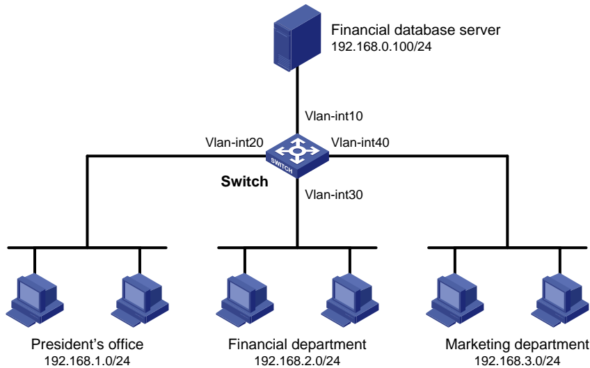
Figure 39 Network diagram
