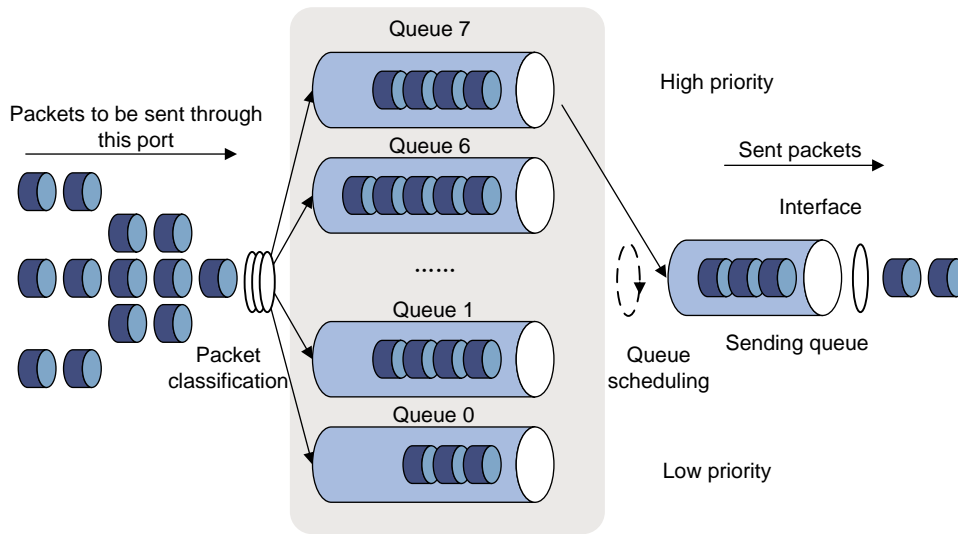
Figure 9 SP queuing
