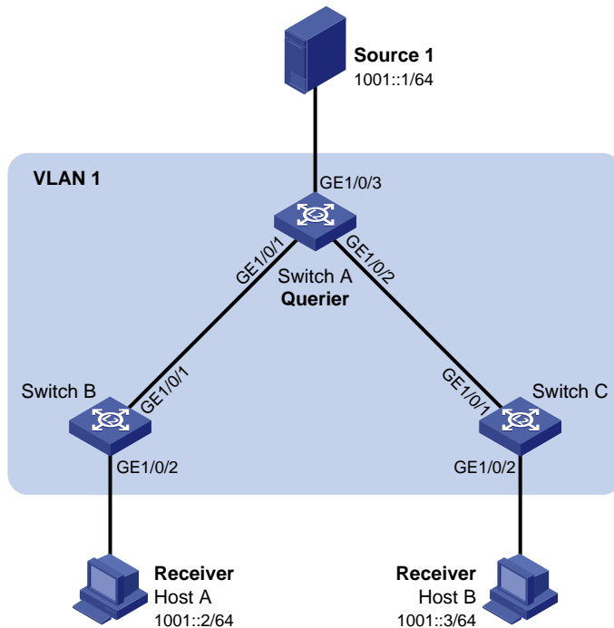
Figure 35 Network diagram
