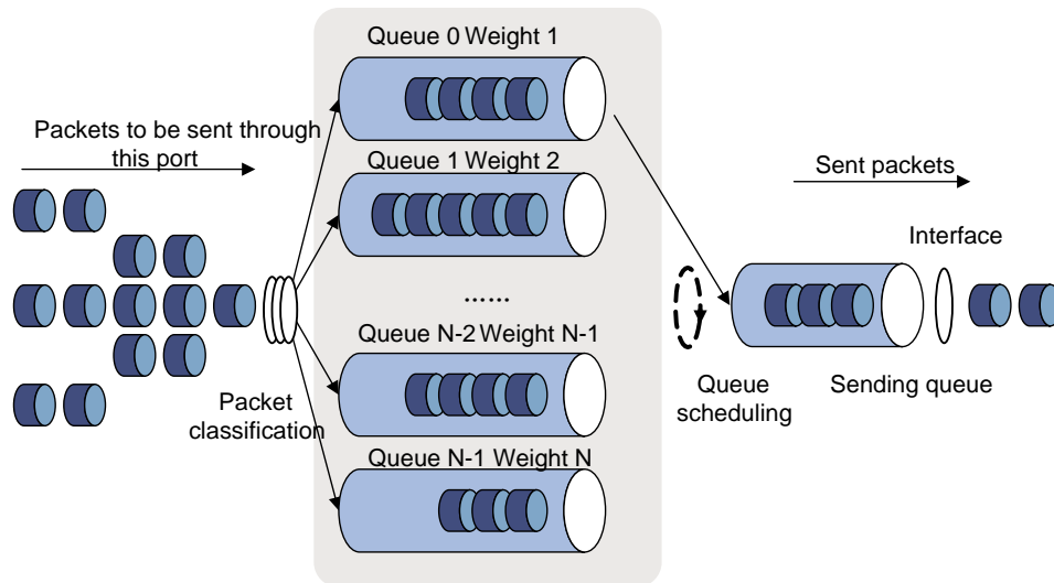
Figure 11 WFQ queuing
